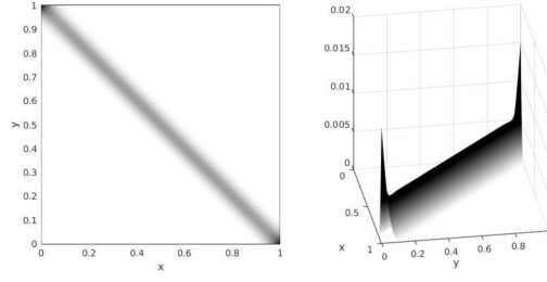
FIGURE 5. Left: support of the optimal coupling. Right: optimal coupling.
