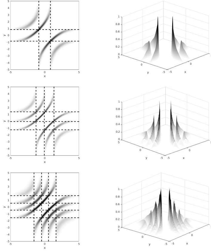
FIGURE 3. (1st Row) Left: support of the optimal coupling \tilde{\gamma}_{12}(x, y) for N = 3 . Right: support of the optimal coupling \tilde{\gamma}_{12}(x, y) for N = 3 (2nd Row) Left: support of the optimal coupling \tilde{\gamma}_{12}(x, y) for N = 4 . Right: optimal coupling \tilde{\gamma}_{12}(x, y) for N = 4 . (3rd Row) Left: support of the optimal coupling \tilde{\gamma}_{12}(x, y) for N = 5 . Right: optimal coupling \tilde{\gamma}_{12}(x, y) for N = 5 . The dashed lines delimit the intervals where \tilde{\mu}_i , with i = 1, \dots, N , are defined.
