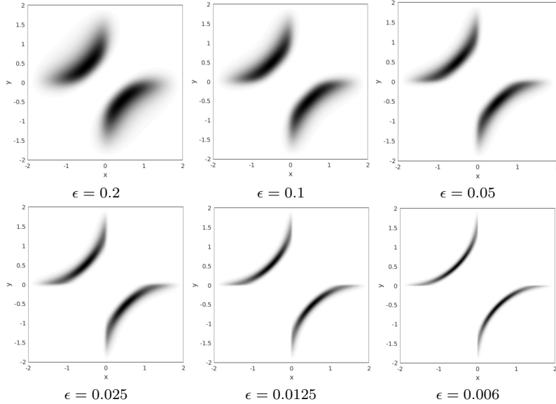
FIGURE 2. Support of the coupling \gamma^\epsilon for the Coulomb cost and all marginals \mu_i = (1+\cos(\pi x/2))/2 . The simulation has been performed on a discretization of [-2, 2] with M_d = 1000 .
