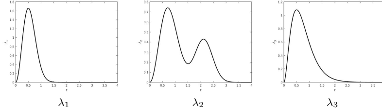
FIGURE 10. Densities \lambda_1 , \lambda_2 and \lambda_3 .
