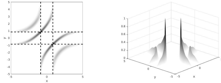
FIGURE 4. (logarithmic cost) Left: support of the optimal coupling \tilde{\gamma}_{12}(x, y) for N = 3 . Right: support of the optimal coupling \tilde{\gamma}_{12}(x, y) for N = 3 . The dashed lines delimit the intervals where \tilde{\mu}_i , with i = 1, \dots, 3 , are defined.
