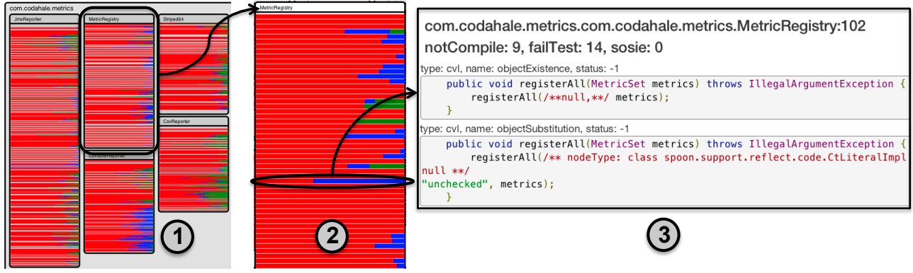
Figure 4: Visualizing the transformations.
