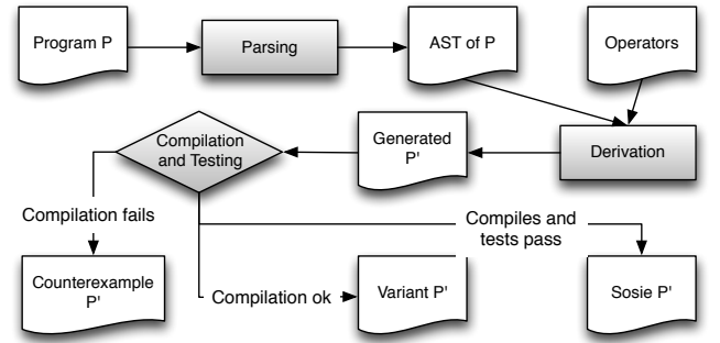
Figure 2: Process to generate variants of Java programs.
