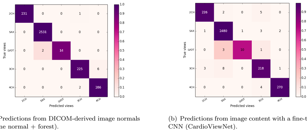
Figure 9. Sum of the confusion matrices over the 10 folds of our crossvalidation on the DETERMINE data-set for the best model classifying images using DICOM normal information and the best image-based predictor (using our fine-tuned neural network).
