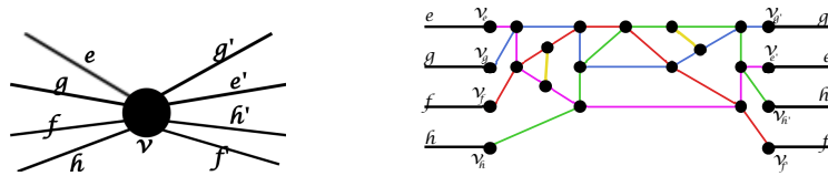
(a) A vertex of degree 8 and allowed transitions A(v) = \{\{e, e'\}, \{e, f'\}, \{f, f'\}, \{f, e'\}, \{g, g'\}, \{g, h'\}, \{h, h'\}, \{h, g'\}\} (edges are ordered as in the planar embedding \mathcal{E} of G ) (b) Gadget D_v : the paths P_{ee'} , P_{ff'} , P_{gg'} , and P_{hh'} are respectively the pink, red, blue and green paths. transitions around vertices v_i , transitions of the paths P_{ee'} , P_{ff'} , P_{gg'} , and P_{hh'} , and transitions containing the yellow edge are allowed
