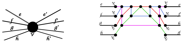
(a) A vertex of degree 8 and allowed transitions A(v) = \{\{e, e'\}, \{f, f'\}, \{g, g'\}, \{h, h'\}\} (edges are ordered as in the planar embedding \mathcal{E} of G ) (b) Gadget D_v : the paths P_{ee'} , P_{ff'} , P_{gg'} , and P_{hh'} are respectively the pink, blue, red and green paths. Transitions around vertices v_i and transitions of paths P_{ee'} , P_{ff'} , P_{gg'} , and P_{hh'} are allowed
