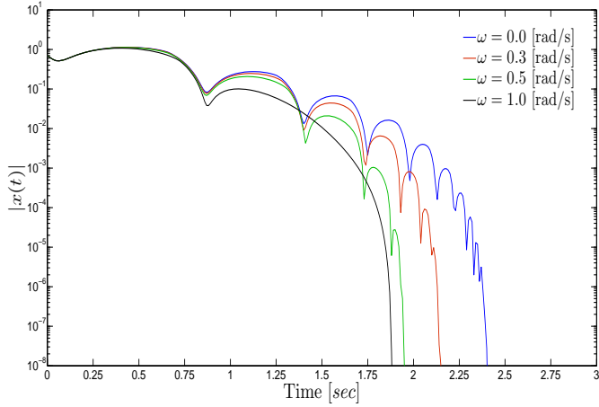
Figure 1. Finite-Time Convergence for Nonlinear Time-Varying System.
