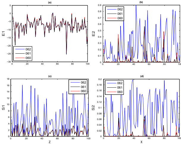
Figure 1: (a), (b) Estimated mean vector and covariance matrix diagonal of the second hidden layer pre-activations, respectively. (c), (d) Estimated mean vector and covariance matrix diagonal of the second hidden layer, respectively.
