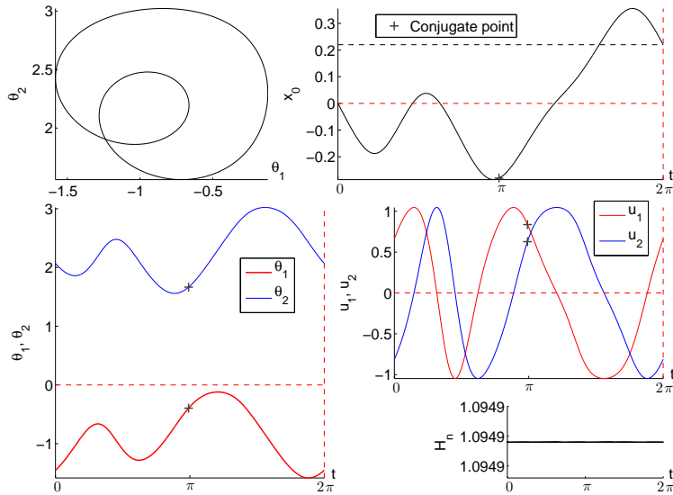
FIGURE 15. Optimal stroke for the f(u_1^2 + u_2^2) cost:limaçon with inner loop. We fixed the displacement to x_0(2\pi) = 0.22 .
