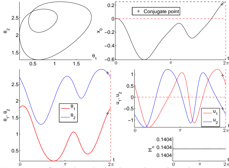
FIGURE 19. Optimal stroke for the mechanical cost:limaçon with inner loop case. We fixed the displacement to x_0(2\pi) = 0.25 .
