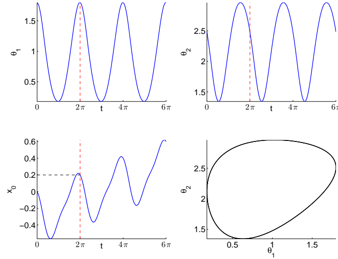
FIGURE 10. A sequence of three identical strokes for the mechanical cost (state variables).
