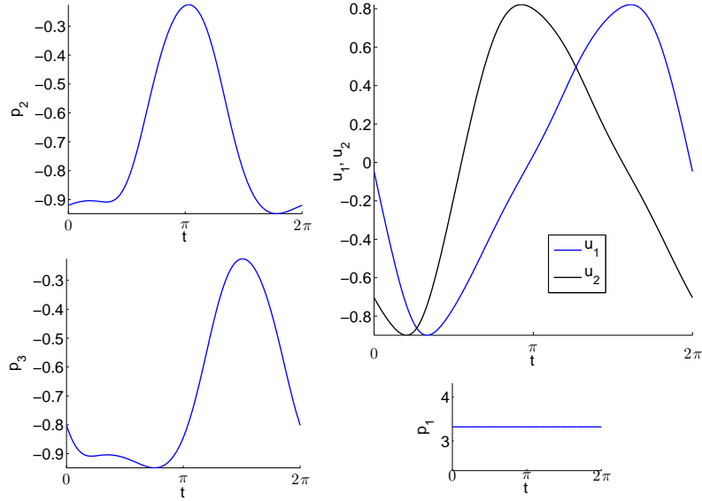
FIGURE 7. Time evolution of the adjoint variables p = (p_1, p_2, p_3) and the control variables u = (u_1, u_2) for the mechanical cost.
