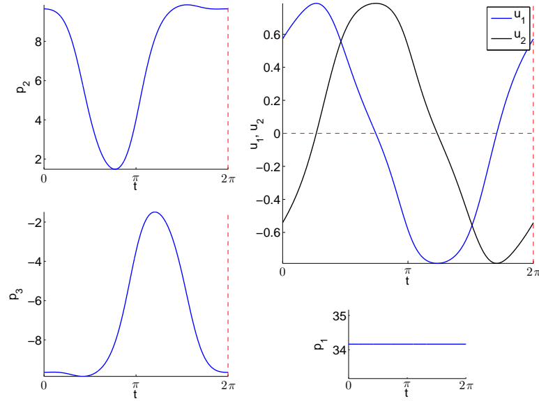
FIGURE 5. Time evolution of the adjoint variables p = (p_1, p_2, p_3) and the control variables u = (u_1, u_2) for the \int (u_1^2 + u_2^2) cost.
