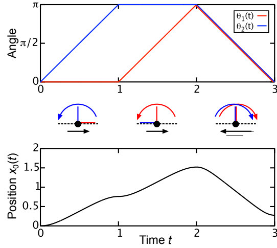
FIGURE 3. Two legs paddling in sequence. The legs perform power strokes in sequence and then a recovery stroke in unison, each stroke sweeping an angle \pi . Arrows show the swimmer and leg velocities at three representative stages of the cycle.
