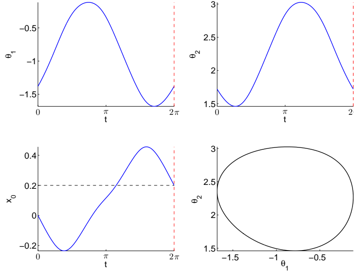
FIGURE 4. Time evolution of the state variables q = (x_0, \theta_1, \theta_2) for the \int (u_1^2 + u_2^2) cost.
