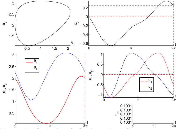
FIGURE 18. Optimal stroke for the mechanical cost:non intersecting case. We fixed the displacement to x_0(2\pi) = 0.25 .
