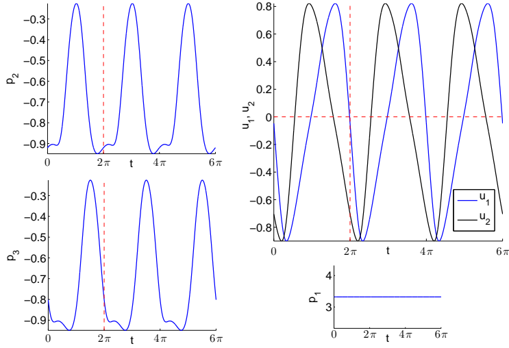
FIGURE 11. A sequence of three identical strokes for the mechanical cost (adjoint variables and control variables).
