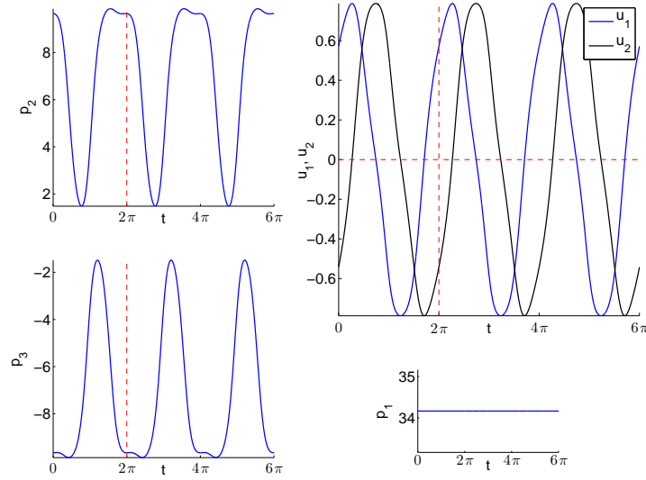
FIGURE 9. A sequence of three identical strokes for the \int(u_1^2 + u_2^2) cost (adjoint variables and control variables).
