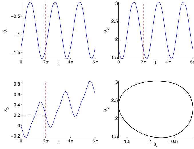
FIGURE 8. A sequence of three identical strokes for the \int(u_1^2 + u_2^2) cost (state variables).
