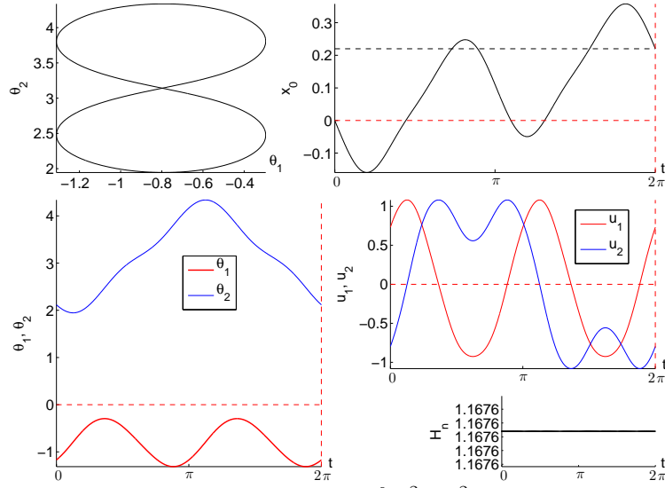
FIGURE 16. Optimal stroke for the f(u_1^2 + u_2^2) cost: eight case. We fixed the displacement to x_0(2\pi) = 0.22 .
