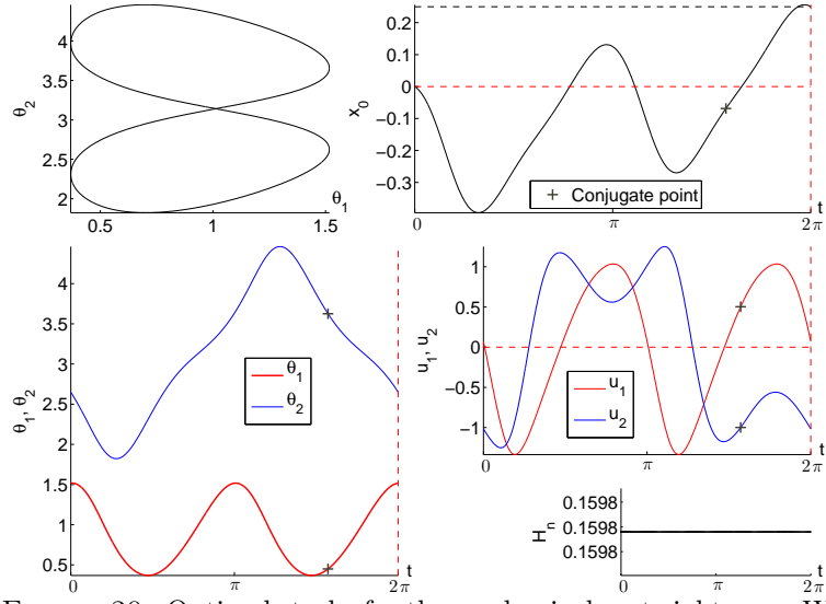
FIGURE 20. Optimal stroke for the mechanical cost: eight case. We fixed the displacement to x_0(2\pi) = 0.25 .
