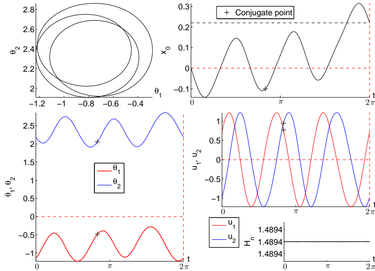
FIGURE 17. Optimal stroke for the f(u_1^2 + u_2^2) cost: multiple self intersections. We fixed the displacement to x_0(2\pi) = 0.22 .
