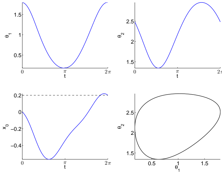
FIGURE 6. Time evolution of the state variables q = (x_0, \theta_1, \theta_2) for the mechanical cost.
