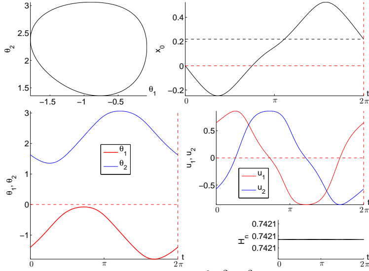
FIGURE 14. Optimal stroke for the f(u_1^2 + u_2^2) cost:non intersecting case. We fixed the displacement to x_0(2\pi) = 0.22 .
