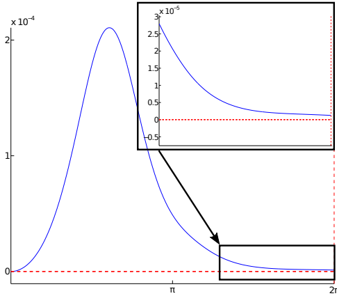
FIGURE 12. Second order sufficient condition checked on a stroke for the \int(u_1^2 + u_2^2) cost. The smallest singular value associated with the rank condition (8) doesn't vanish on ]0, 2\pi] , and there is no conjugate time.
