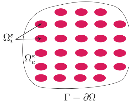
Figure 1: The domain \Omega = \overline{\Omega}_e^\varepsilon \cup \Omega_i^\varepsilon containing positive and negative materials.
