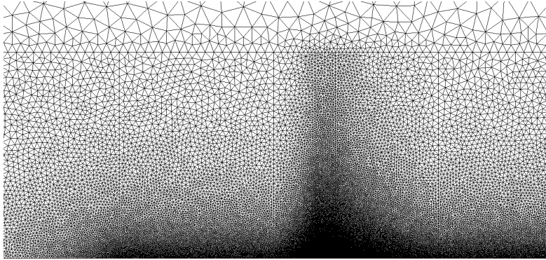
Figure 22: Jet case: mesh
