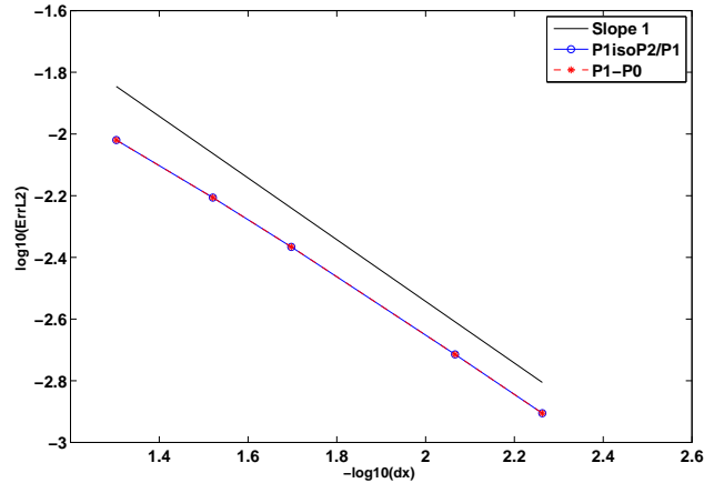
FIGURE 5. Convergence rate of the solitary wave solution for \mathbb{P}_1/\mathbb{P}_0 and \mathbb{P}_1 -iso- \mathbb{P}_2/\mathbb{P}_1 scheme.
