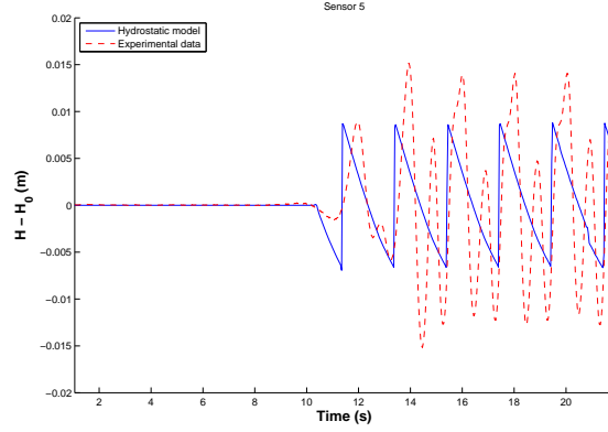
FIGURE 9. Comparison with hydrostatic model on sensor 5.
