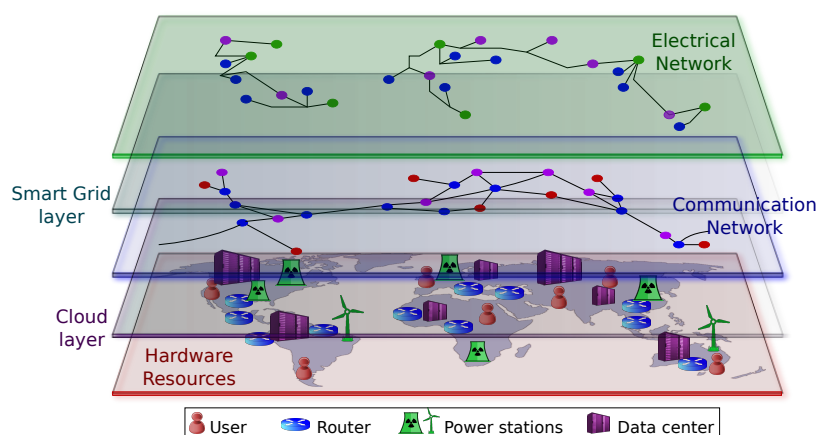
Figure 1: Representation of the involved resources and layers on the example of a worldwide Cloud
