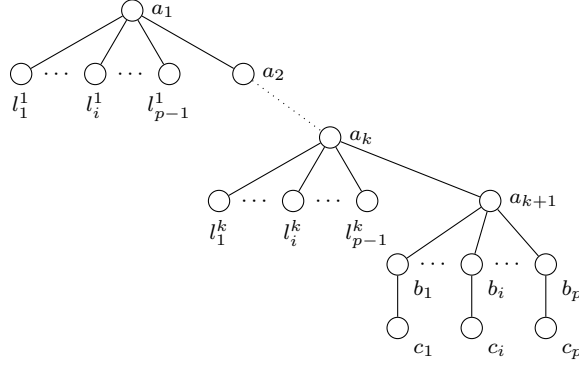
Fig. 7. No memory bound for PARSUBTREESOPTIM.
