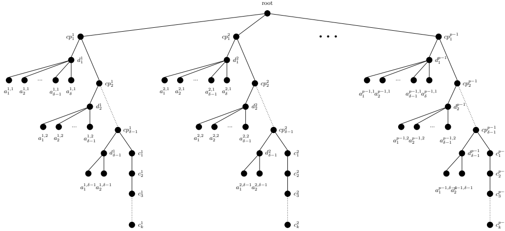
Fig. 4. Tree used for establishing Theorem 4.6.
