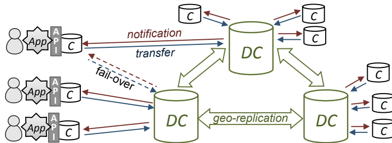
Figure 1: System components ( A pplication processes, C lients, D Cs), and their interfaces.
