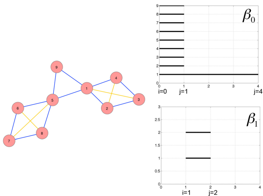
Fig. 1 Example of Betti number calculation for a simple network. A simple network with red nodes and blue edges consists of two four-node cycles connected via a three-node cycle (Panel a). The Betti number algorithm adds the yellow edges in calculation of filtration index effectively “killing” the four-node cycles by eliminating the cycles. The numerical value for the Betti number is the number of bars lasting from index i to index j in a Betti barcode. Each bar starts when a homology class is born and ends when this class is killed due to appearance in the filtration of a higher dimensional chain whose boundary is the underlying cycle. Thus, Betti0 is equal to 9 and represents the number of nodes (Panel b), and Betti1, is equal to 2, and represents the number of rings of four nodes (Panel c)
