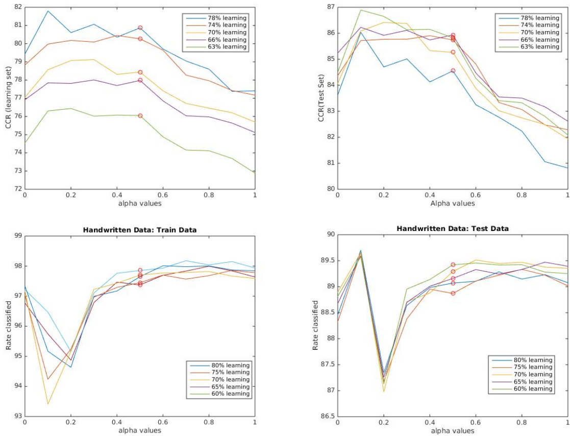
Figure 2: Correct Classification Rate (CCR) obtained with Sylla & Girard kernel (4, 5) for \alpha \in \{0, 0.1, \dots, 1\} and several proportions \tau . The results obtained with the RBF kernel ( \alpha = 0.5 ) are emphasized by a red circle. Left: CCR computed on the learning set, Right: CCR computed on the test set. Top: results obtained on the verbal autopsy data, bottom: results obtained on the handwritten digit data.
