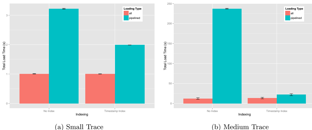
FIGURE 13 – Total Gantt Chart load time for small and medium traces, using different loading types, and using or not timestamp indexing.
