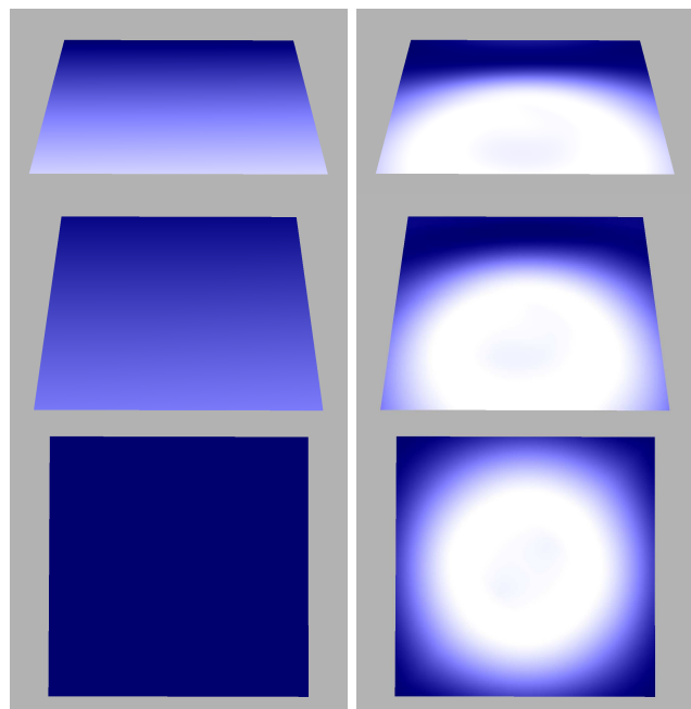
Fig. 6 Toy example generalizing Fig. 2: four radiance functions are stored on a four-vertex plane. Their normals diverge and the functions represent a diffuse + specular behavior ( i.e. , a Phong-like BRDF). Left (naive interpolation): the specular highlight fades out at some angles. Right (equation (8)): the specular highlight is well interpolated.
