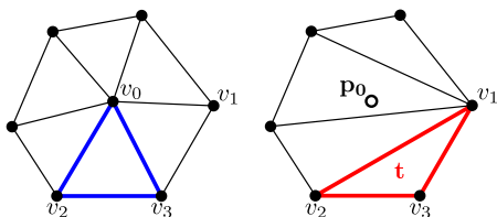
Fig. 3 Half-edge collapse of v_0v_1 onto v_1 . The point \mathbf{p}_0 (position of the vertex v_0 before collapse) is generally off the surface after collapse.
