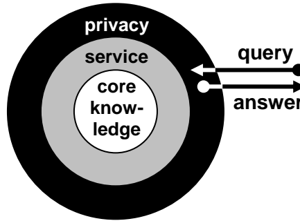
Figure 3 Three-layer architecture
