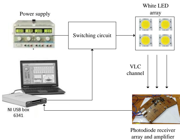
Fig. 20: Experimental setup.
