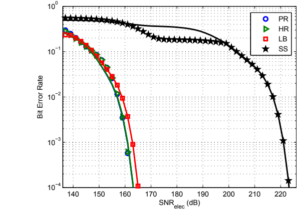
Fig. 17: BER as a function of \text{SNR}_{\text{elec}} of the PR, HR, LB and SS receivers at Position 0 with simulation curves (lines) and analytical curves (markers) for d_{\text{tx}} = 3 m.
