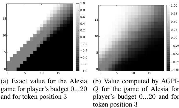
Figure 2. Value functions at token position 3
