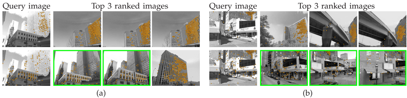
Fig. 8. Examples of place recognition results on the Pittsburgh dataset. Each figure shows the query image (left column) and the three best matching database images (2nd to 4th column) using the baseline burstiness method [8] (top row) and the proposed reptile detection and adaptive assignment (bottom row). The green borders indicate correctly recognized images. The orange dots show the visual word matches between the query image (1st column) and the best matching database image (2nd column). The visual word matches are also displayed on the 2nd and 3rd best matching images. Please note that for improved clarity, the matching visual words in the query are not shown for the second and third match.
