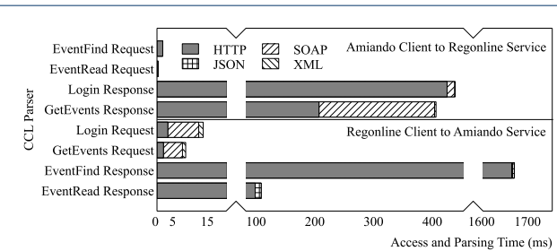
Figure 10: Access & Parsing time decomposed by Atomic parsers
