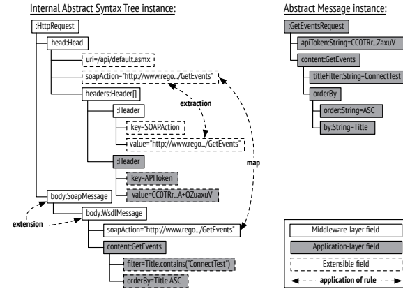
Figure 7: AST of Regonline GetEvents-Request
