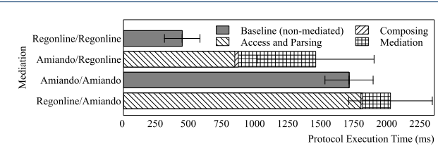
Figure 9: Comparison between mediated and non-mediated executions
