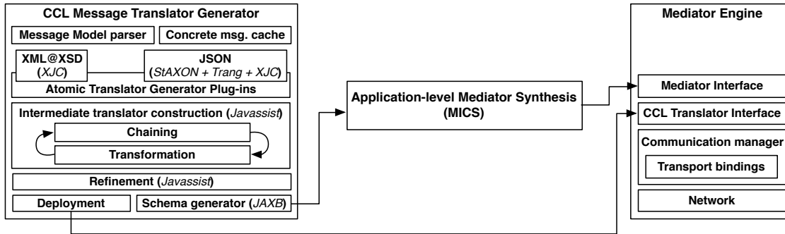
Figure 8: Implementation of the unified mediation framework
