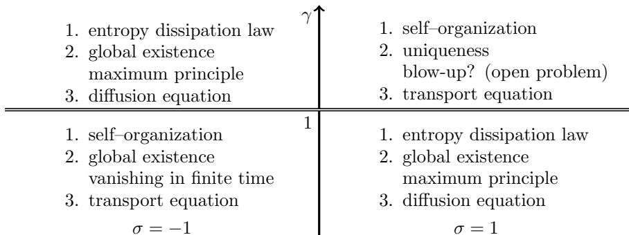
FIGURE 1. Properties accordingly to the parameters \sigma and \gamma .
