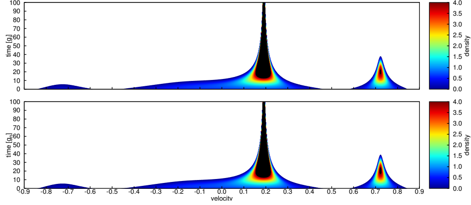
FIGURE 4. Numerical result of the negative gregarious interaction case, i.e. \sigma = -1 , \gamma = 0.5 . Semi-implicit scheme (15) [g_i] (first line), and non-linear scheme (19) [g_n] (second line).
