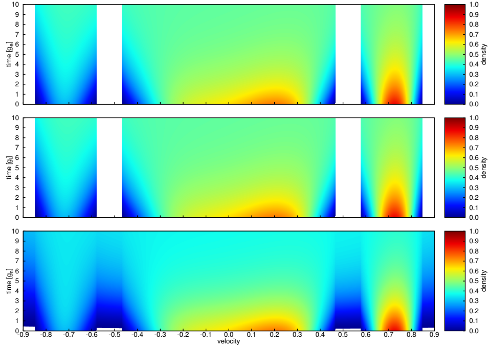
FIGURE 3. Numerical result of the positive solitarious interaction case, i.e. \sigma = 1 , \gamma = 0.5 . Explicit scheme (13) [g_e] (first line), semi-implicit scheme (15) [g_i] (second line), and nonlinear scheme (19) [g_n] (third line).
