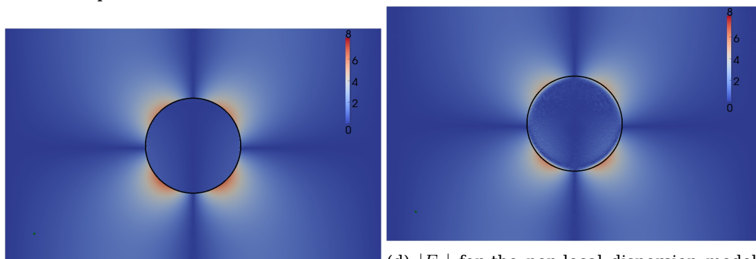
(c) |E_y| for the local Drude model. The surface plasmon mode is clearly observable. Although the local model allows a penetration, it is hardly seeable due to the very short penetration depth.
