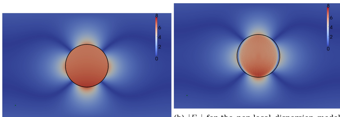
(a) |E_x| for the local Drude model. The surface plasmon mode is clearly observable. Although the local model allows a penetration, it is hardly seeable due to the very short penetration depth.
