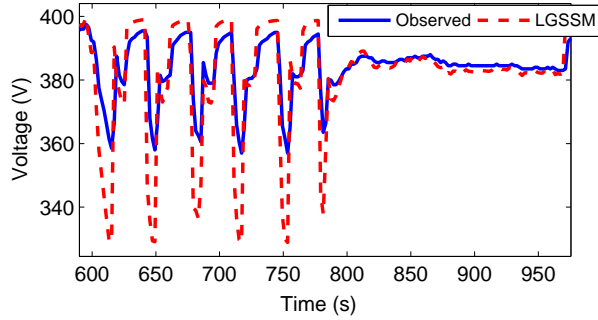
Figure 14: [Real data] Prediction of the voltage using a linear Gaussian state-space model
