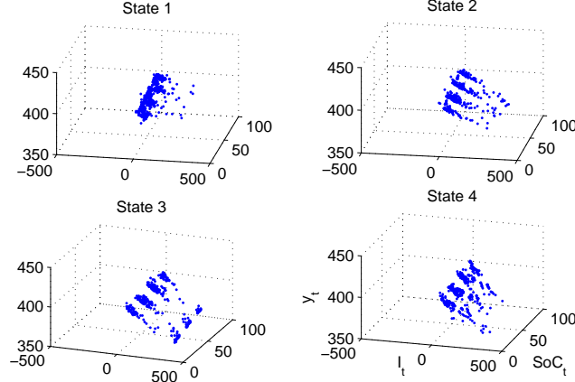
Figure 17: [Real data] Voltage vs \text{SoC} vs current: instantaneous measurements under each hidden Markov state for a SMSSM with \kappa = 4
