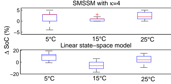
Figure 16: [Real data] Difference between Coulomb counting and estimated \text{SoC} using SMSSM with \kappa = 4 (top) and Linear state-space model (bottom) for ambient temperature equal to 5, 15, 25°C
