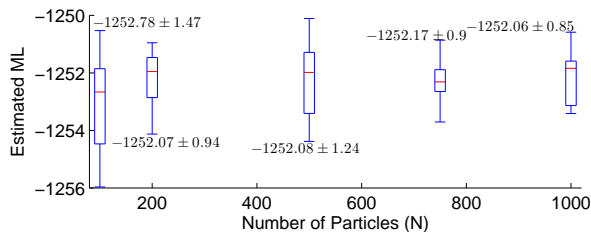
Figure 7: [Simulated data] Estimated ML for N = \{100, 200, 500, 750, 1000\} with \kappa = 5 ; 20 different initializations of the EM algorithm for each case
