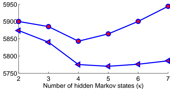
Figure 15: [Real data] BIC (o) and AIC ( \Delta ) with \kappa = \{2, \dots, 7\}
