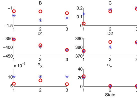
Figure 8: [Simulated data] Comparison between true (*) and estimated (o) parameters with \kappa = 3
