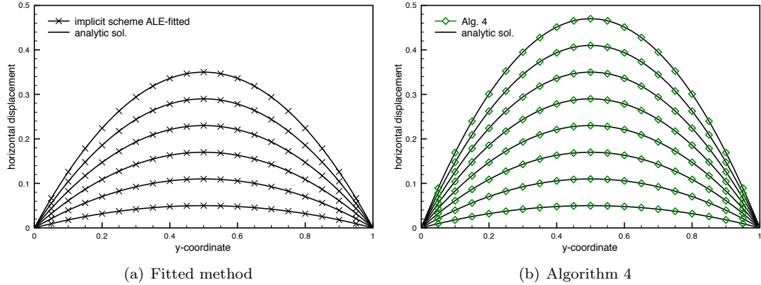
Figure 20: Displacements at steady state for increasing inlet pressures.
