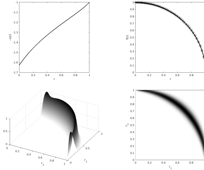
Fig. 5 Top-Left: Kantorovich Potential v(r) . Top-Right: Numerical co-motion function (solid line) and analytical co-motion (star-solid line) . Bottom-Left: Transport plan \tilde{\gamma} . Bottom-Right: Support of \tilde{\gamma} .
