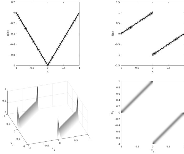
Fig. 4 Top-Left: Kantorovich Potential u(x) . Top-Right: Numerical co-motion function (solid line) and analytical co-motion (star-solid line). Bottom-Left: Transport plan \tilde{\gamma} . Bottom-Right: Support of \tilde{\gamma} .
