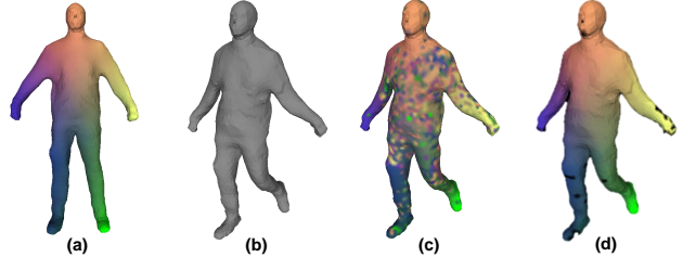
Figure 7. (a) references surface of S2 (vertex indices encoded with colors). (b) test mesh. (c) matching results with MeshHOG. (d) matching results of the proposed VNF-forest framework.
