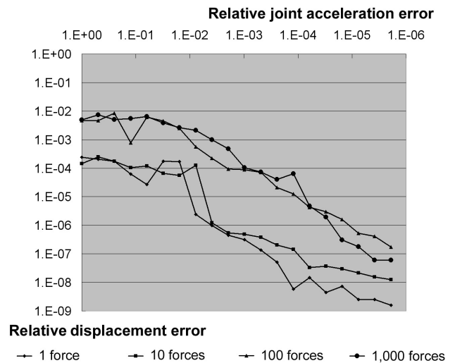
Figure 8: Influence of the relative joint acceleration error on the relative displacement error. As the precision enforced on the computation of the joint acceleration increases, the precision in the final configuration of the linkage expressed in the world frame increases as well.
