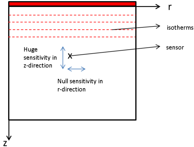
Figure 26: Simple 1D heating, showing the horizontal isothermal lines; there is a null sensitivity along the r -axis.
