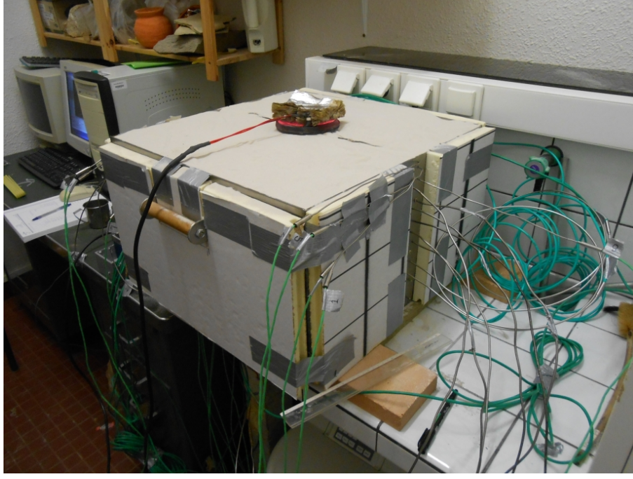
Figure 15: Experimental hearth.
