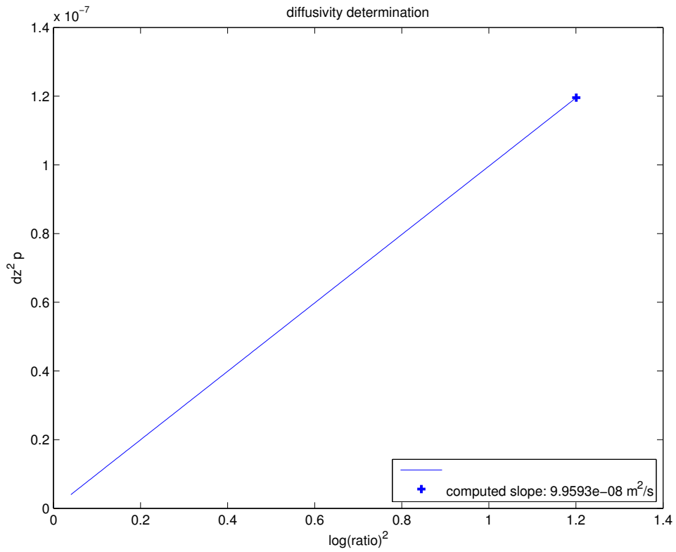
Figure 21: Diffusivity Determination
