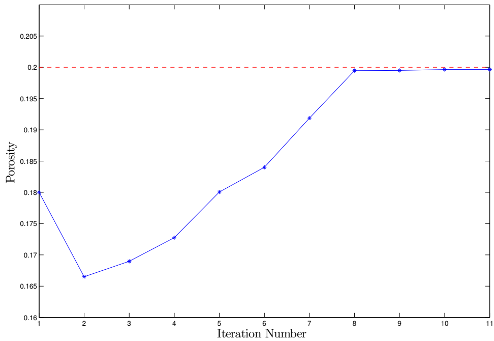
Figure 6: Variation of the porosity as function of iteration number using LMA (Same number of mesh cells in both the forward and inverse problems). The red line represents the exact value of \phi .
