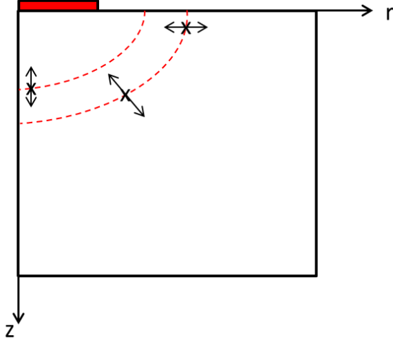
Figure 27: In a 3D-axi heating, the isothermal lines are very close to ellipsoidal curves; there is a null sensitivity in a direction normal to these curves.
