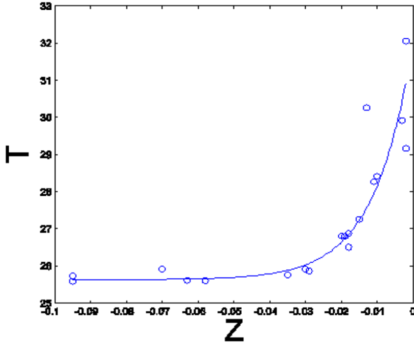
Figure 30: Initial temperature profile of the second experiment, showing that the temperature is not uniform; however a fit to an exponential law works quite well.
