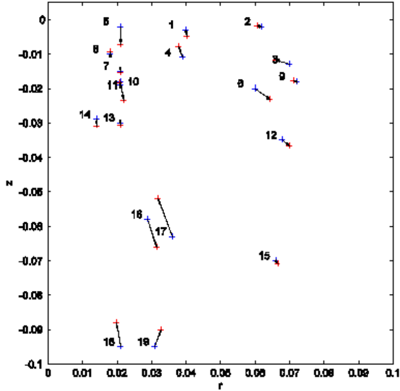
Figure 31: Displacement of the sensors after solving the inverse problem, for the second experiment.
