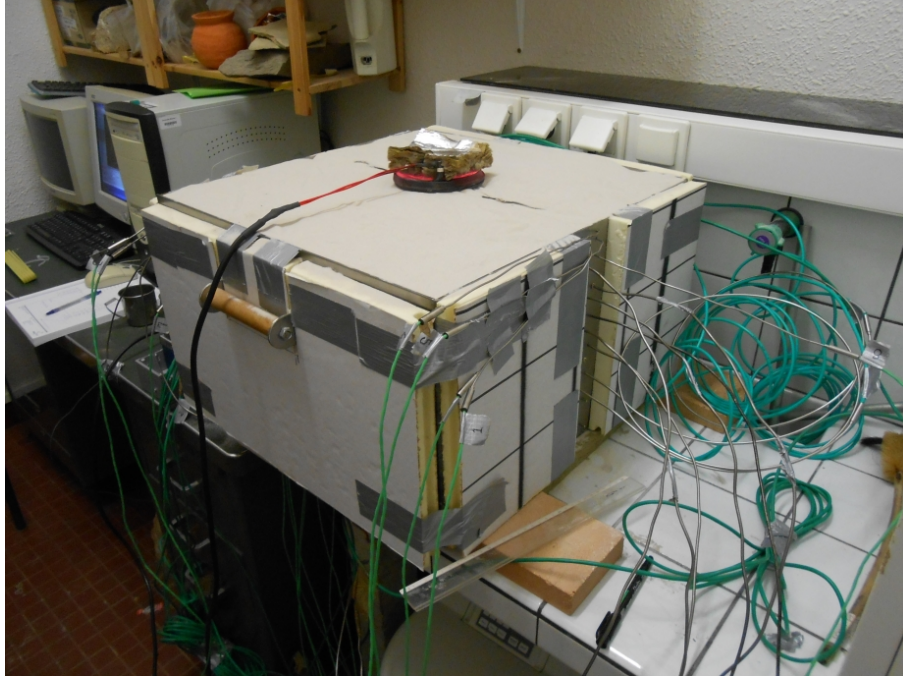
Figure 14: Experimental hearth.
