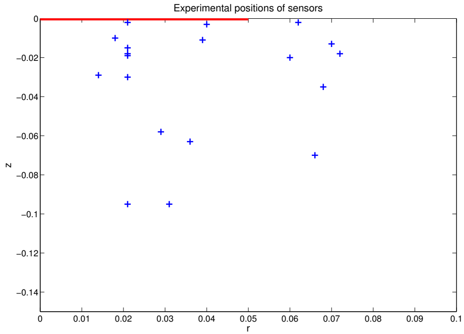
Figure 33: Experimental positions of 19 sensors in blue. The red bar represents the fire (unit is meter for both axes).
