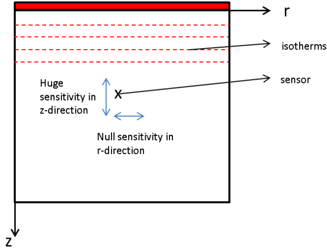
Figure 25: Simple 1D heating, showing the horizontal isothermal lines; there is a null sensitivity along the r -axis.
