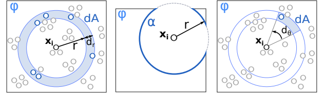
Figure 3: Left: Radial density function. For a point x_i and a radius r = kd_r , we count the number of points within a range of distances d \in [kd_r, (k+1)d_r] of x_i . Center: Window-edge effect correction. We evaluate \alpha as the circumference of circle C(x_i, r) that intersects the active region \varphi . This value is used to normalize the integration region dA . Right: Oriented radial density function. The range is reduced to points with an angle ranging in d_\theta \in [ld_\omega, (l+1)d_\omega] .
