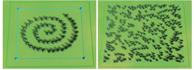
Figure 17: An example of a failure case. The spiral arrangement of trees (left) cannot be reproduced by our system (right), since we only capture pairwise distributions of distances and orientations.
