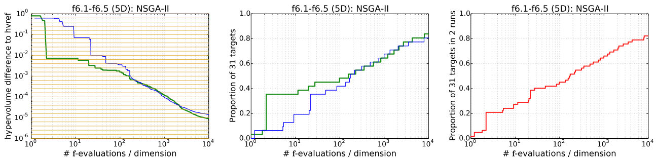
Figure 1: Recovery of convergence graphs using data profiles. The left plot shows the difference over time between the hypervolume indicator in two runs of NSGA-II to the hypervolume of the reference set on a combination of two instances (1 and 5) of the Attractive Sector function ( f_6 ) in 5- D . The middle plot shows the corresponding data profile for each run individually using the 31 target values displayed as light (brown) horizontal lines on the left plot. The right plot shows the data profile, aggregated over the two runs.
