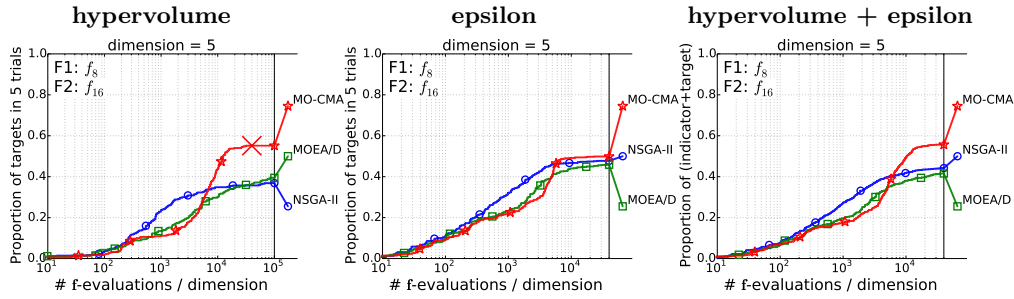
Figure 6: Data profiles of algorithm performances for the combination of Rosenbrock ( f_8 ) and Weierstrass ( f_{16} ) functions in 5-D. The left and center plots show data profiles for the hypervolume and \varepsilon -indicator respectively, and the right plot shows the aggregation over both indicators.
