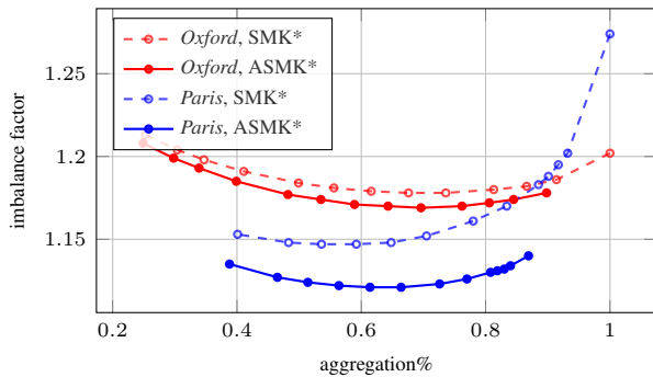
Figure 10. SMK*/ASMK* imbalance factor vs. aggregation% on Holidays-L . Vocabulary size k = 65k ; selectivity exponent \alpha = 3 .
