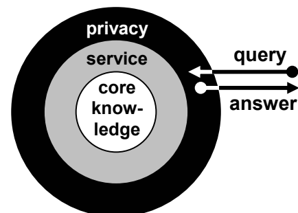
Figure 3 Three-layer architecture
