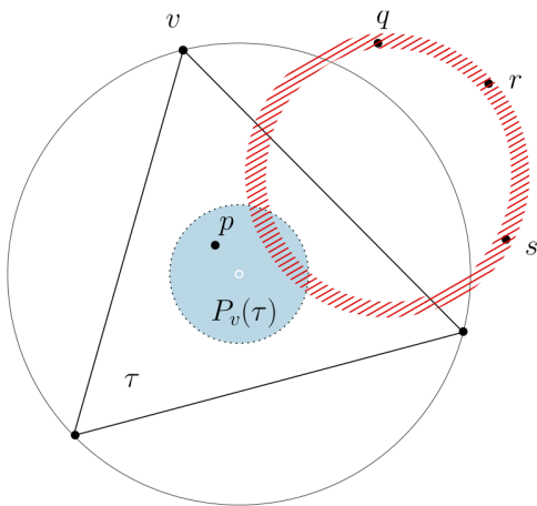
Fig. 3. The picking region of triangle \tau . Set \sigma = \{q, r, s\} is a hitting set for the picking region P_v(\tau) . It defines a forbidden region, shown with red dashes, to be avoided by the refinement point p of \tau .
