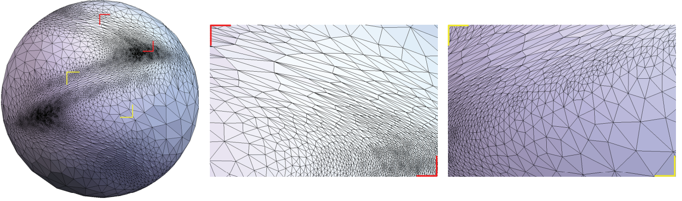
Fig. 4. A unit sphere endowed with a metric field derived from the sine-shaped shock function E(x, y, z) = \tanh(\frac{1}{\lambda}(2x - \sin(5y))) + x^3 + xy^2 . \lambda = 0.6 , \rho_0 = 3.0 , r_0 = 0.1 , \gamma_0 = 1.4 , \beta = 2.5 and \delta = 0.3 . The mesh has 18323 vertices and 36642 facets.
