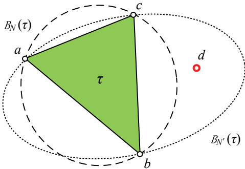
Fig. 2. The configuration (\tau, d) is quasi-cospherical because point d is outside the N -circumball B_N(\tau) but inside the N' -circumball B_{N'}(\tau) .
