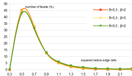
Fig. 10. Squared radius-edge ratios in meshes obtained with different values of \beta and \delta .
