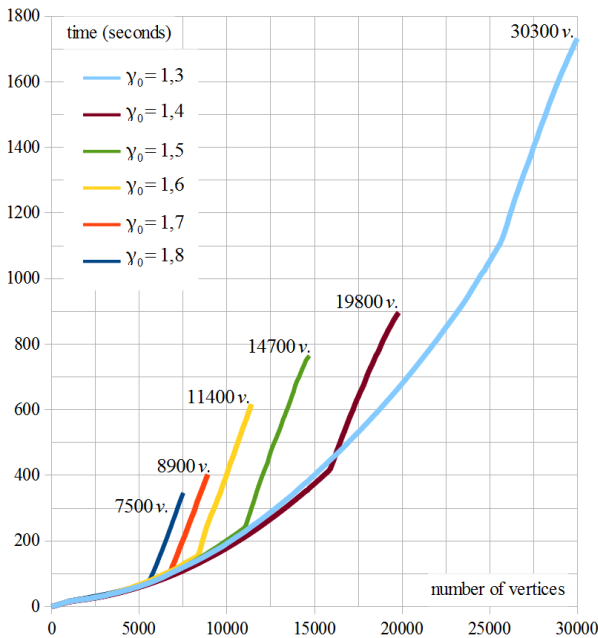
Fig. 7. Computing time to mesh an implicit torus with r_0 = 0.1 and different values of \gamma_0 between 1.3 and 1.8.
