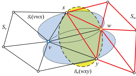
Fig. 1. Example of inconsistent stars in 2D : stars S_v and S_w are inconsistent because edge [vw] belongs to S_v but not to S_w .
