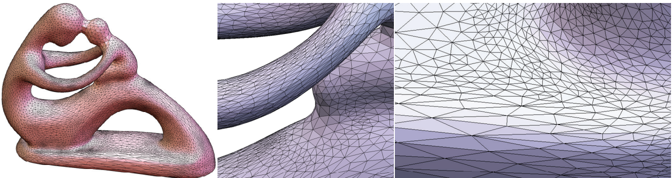
Fig. 6. Result on the polyhedral surface “fertility”, a model from AIM@SHAPE repository. We took r_0 = 0.1 , \gamma_0 = 1.5 . The mesh has 12,480 vertices and 24,972 facets.
