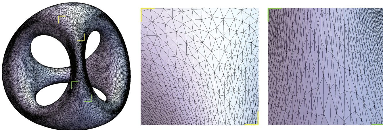
Fig. 5. The “chair” implicit surface with a curvature-related metric field. The equation of the chair is f(x, y, z) = (x^2 + y^2 + z^2 - ak^2)^2 - b((z - k)^2 - 2x^2)((z + k)^2 - 2y^2) . In this example, a = 0.8 , b = 0.4 , k = 1.0 , \rho_0 = 3.0 , r_0 = 0.1 , \gamma_0 = 1.3 , \beta = 2.5 and \delta = 0.3 . The mesh has 24164 vertices and 48336 facets.
