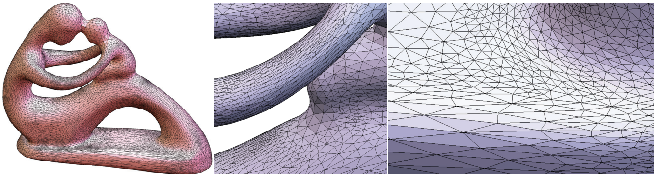
Fig. 6. Result on the polyhedral surface “fertility”, a model from AIM@SHAPE repository. We took r_0 = 0.1 , \gamma_0 = 1.5 . The mesh has 12,480 vertices and 24,972 facets.
