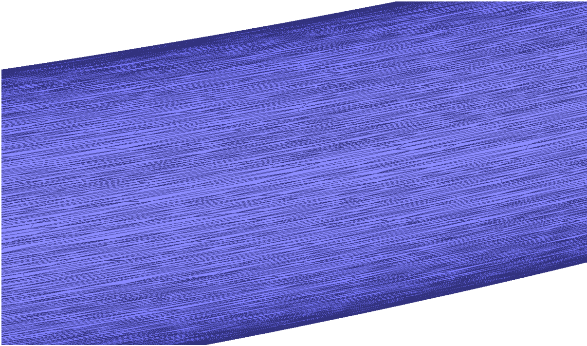
Fig. 9. Anisotropic Delaunay mesh of a piece of torus with big radius 50 and small radius 1. We took \rho_0 = 3.0 , \gamma_0 = 1.8 , r_0 = 1.0 , \beta = 2.5 , \delta = 0.3 . The approximation error is smaller than 0.001.
