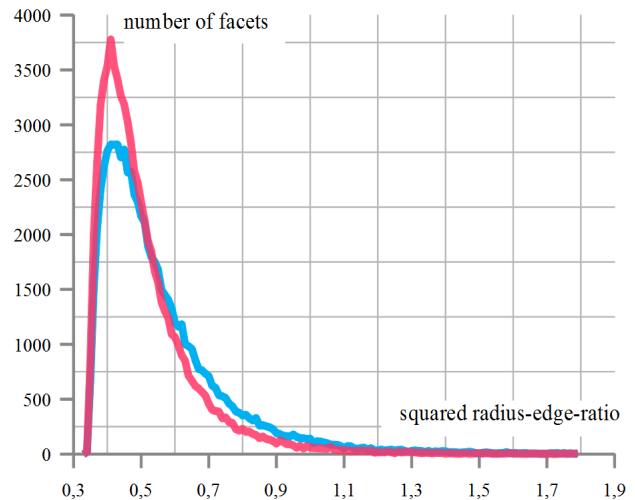
Fig. 8. The distributions of the squared radius-edge ratios of the mesh facets, respectively before (blue curve) and after (red curve) the optimization step. The radius-edge ratio of each mesh facet is computed three times, using each time the metric attached to one of the three vertices. Model: “fertility”, r_0 = 1.0 , \gamma_0 = 1.5 .
