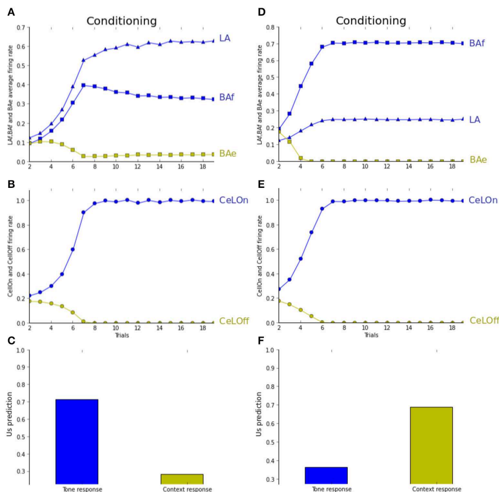
FIGURE 5 | (A–C) Pairing experiment (see text for details). (D–F) Pairing experiment with increased ACh level. (B,E) CeLON activity increases, and correctly predicts US arrival after a few trials in both experiments. (A) LA (blue triangles) and BAf (blue squares) activities increase during training. BAe activities (green squares) weakly decrease due to inhibition. Starting from trial 6, BAf activities are weakly decreasing due to the reduction of uncertainty, which reduces ACh. (C) CeLON activity after learning, when only the tone CS (blue bar) or only the context (green
