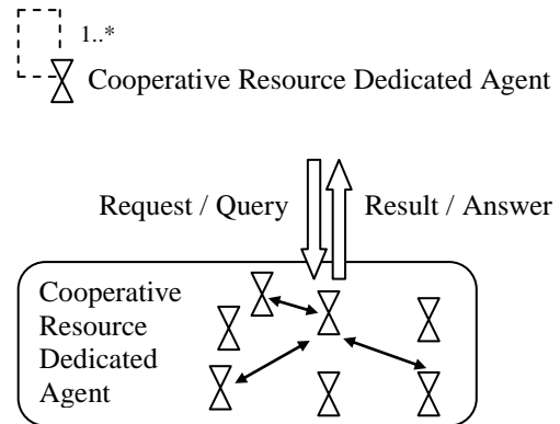
Figure 10. Peer-to-peer sub-society
