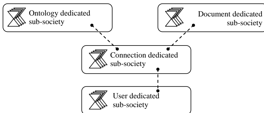
Figure 8. Identified Sub-Societies
