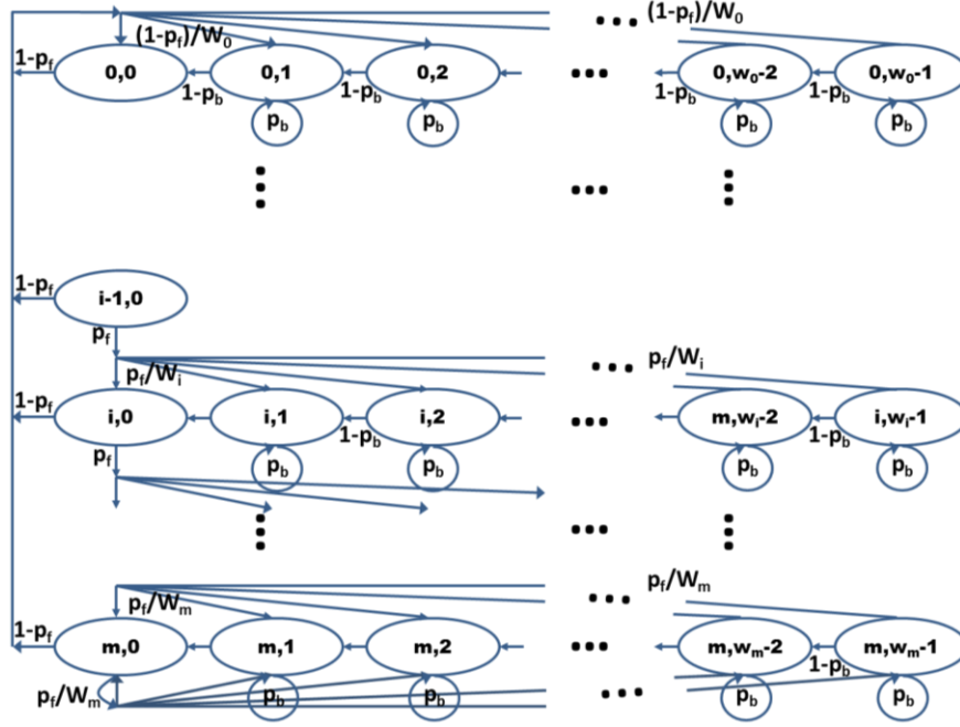
Figure 9: Markov model of the back off procedure. Rows indicate the stage of the back off, while columns represent the state of the back off counter.
