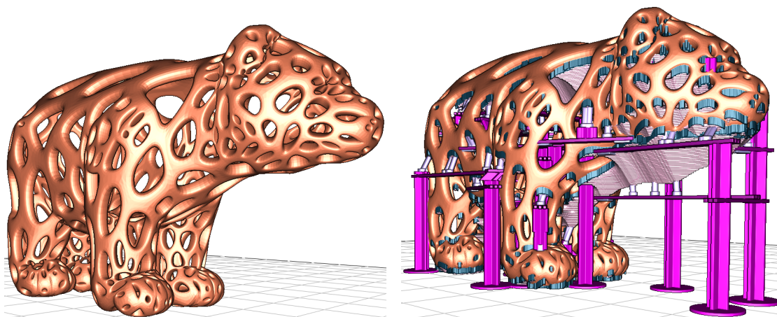
Figure 15: The support structure for the bear model.
