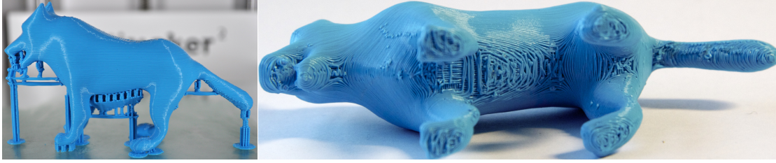
Figure 12: The wolf . Side view with our support structure and bottom view with support removed. The quality is equivalent to standard single-material support techniques.
