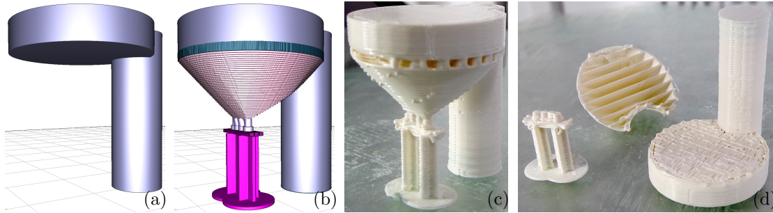
Figure 9: (a) A toy example printed in the worst orientation for illustration. (b) In blue, the crust; in purple, the enclosure supporting the crust; below, the scaffolding. (c) The resulting print on the Ultimaker 2 bed. (d) The supporting structure has been detached from the object. Note how only two pillars are required, since the enclosure reduces in volume as quickly as possible while being printable.
