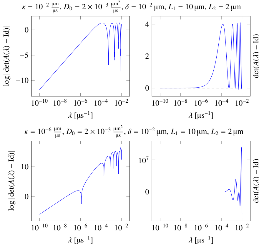
Figure 3: Evolution of \det(A(\lambda) - \text{Id}) in logarithmic (left) and natural scale (right) for L_{\text{extra}} = 2 for the semi-permeable membrane.
