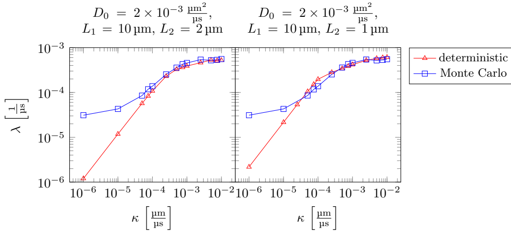
Figure 5: Deterministic and probabilistic estimation of the smallest positive eigenvalue for several values of \kappa .
