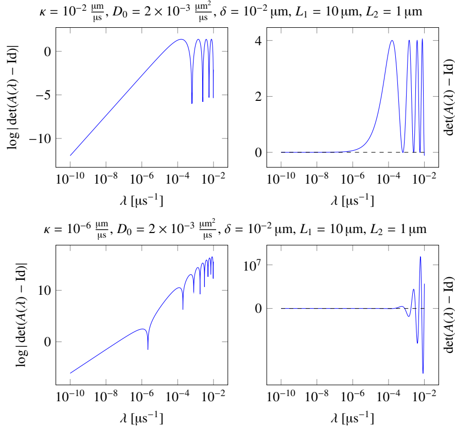
Figure 4: Evolution of \det(A(\lambda) - \text{Id}) in logarithmic (left) and natural scale (right) for L_{\text{extra}} = 1 for the semi-permeable membrane.
