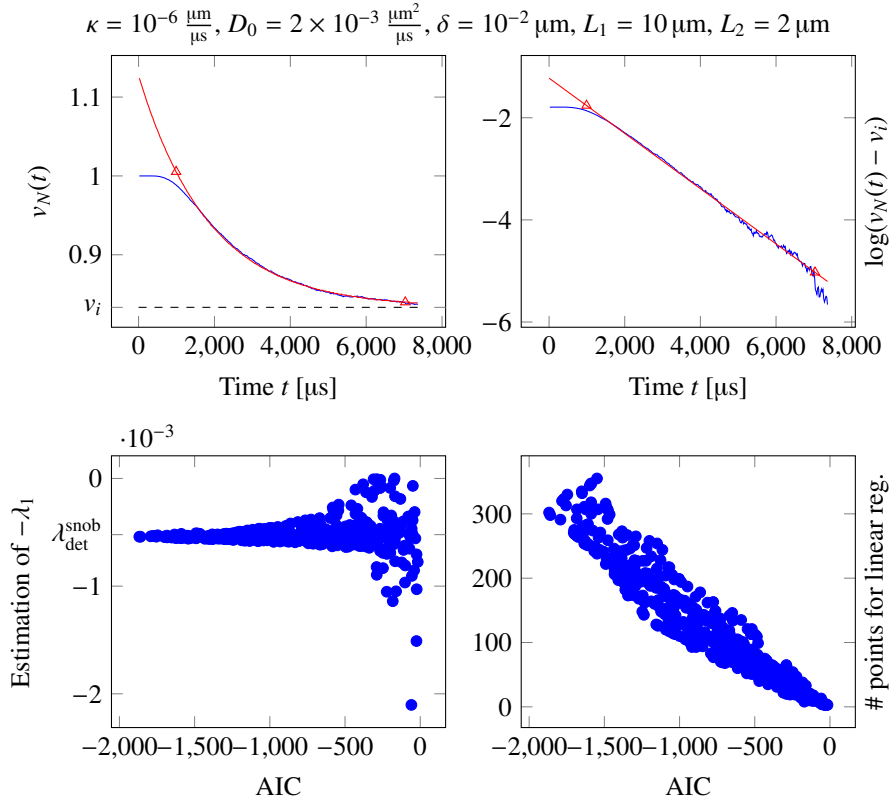
Figure 2: Evolution of the concentration in the intra-cellular domain and estimation of the smallest positive eigenvalue.
