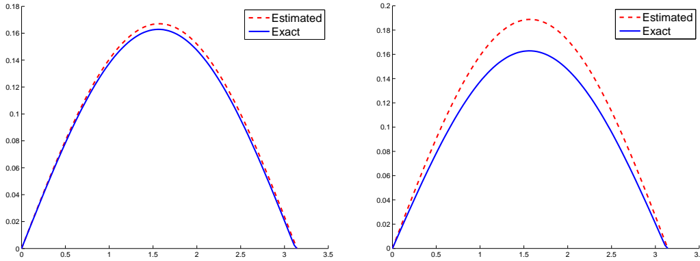
FIGURE 11. Estimated (dashed line) and exact total population at time t = T with 5% of noise (left) and 15% of noise (right).
