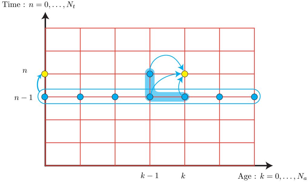
FIGURE 3. Step n of the algorithm. The unknown \mathbf{U}^{n,k} at each node (k, n) is the vector containing the solution at the different points of the space discretization.
