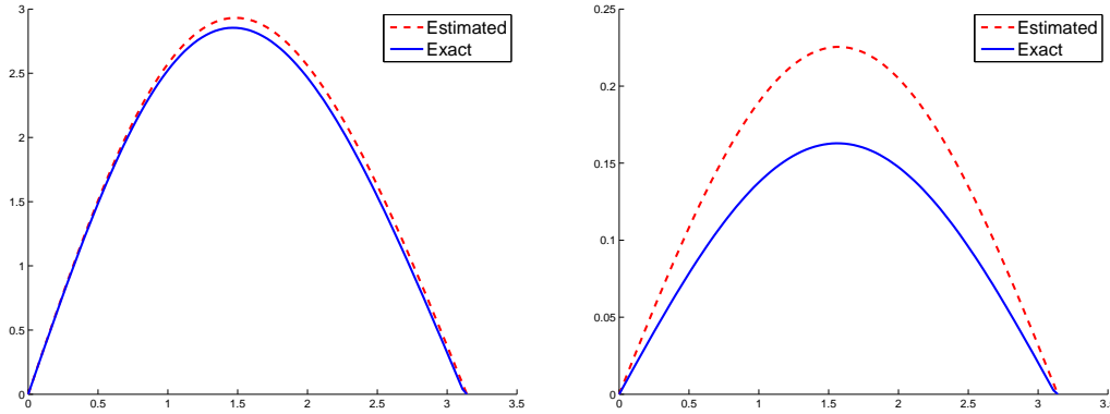
FIGURE 12. Estimated (dashed line) and exact total population at time t = T with age observation near a = 0 (left) and far from a = 0 (right).
