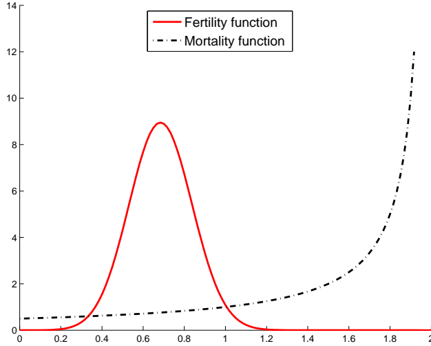
FIGURE 5. The fertility and mortality functions.
