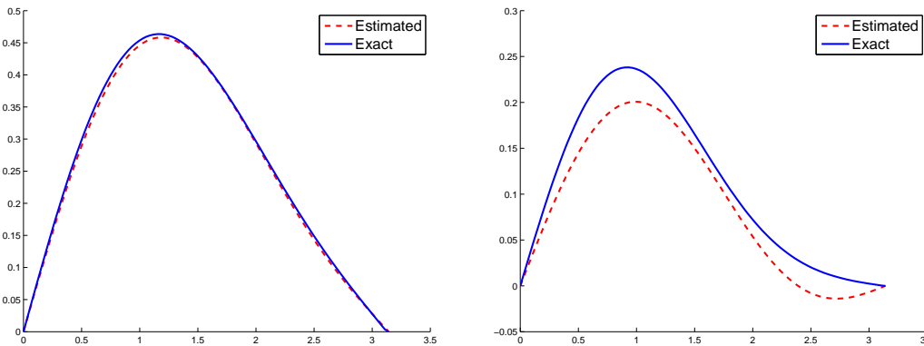
FIGURE 13. Estimated (dashed line) and exact total population at time t = T , for T = a^* (left) and for T = 0.5a^* (right).
