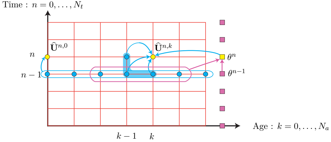
Figure 4: Step n of the algorithm. First, \theta_i^n is computed using \theta_i^{n-1} and \widehat{\mathbf{U}}^{n-1,k} , for k = N_{a_1} - 1, \dots, N_{a_2} (pink arrows). Next, \widehat{\mathbf{U}}^{n,0} is deduced from \widehat{\mathbf{U}}^{n-1,k} , for k = 0, \dots, N_a . Finally, \widehat{\mathbf{U}}^{n,k} for k \geq 1 is computed using \theta_i^n , \widehat{\mathbf{U}}^{n,k-1} , \widehat{\mathbf{U}}^{n-1,k} and \widehat{\mathbf{U}}^{n-1,k-1} (blue arrows).
