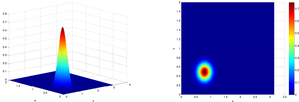
Figure 8: Gaussian initial state (3D and 2D representations).
