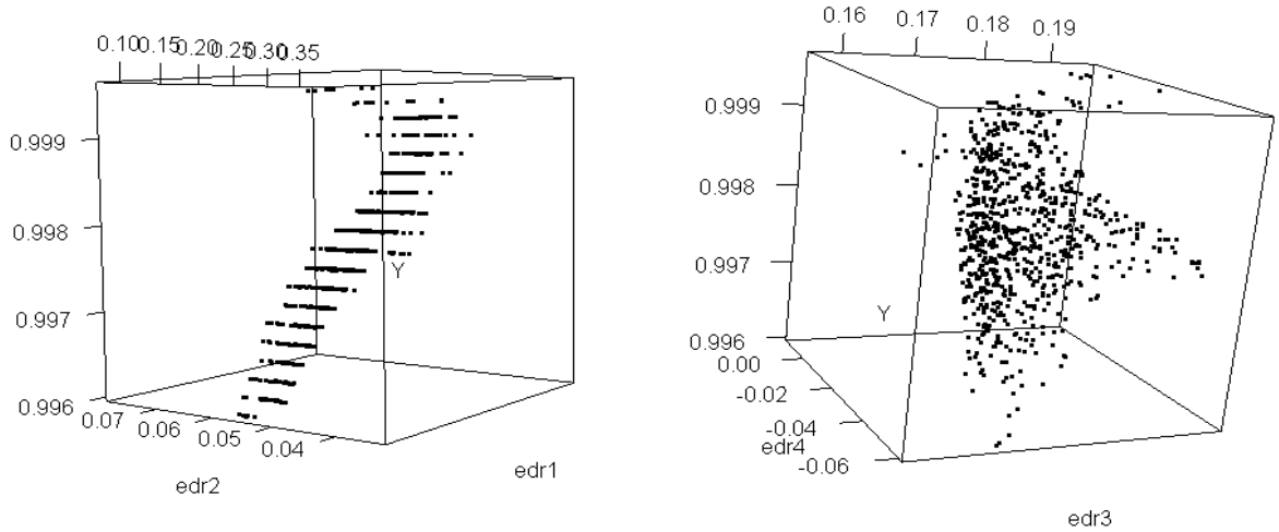
Figure 9: 3D-plot of the dependent variable versus the first two EDR indices (on the left); 3D-plot of the dependent variable versus the third and fourth EDR indices (on the right)
