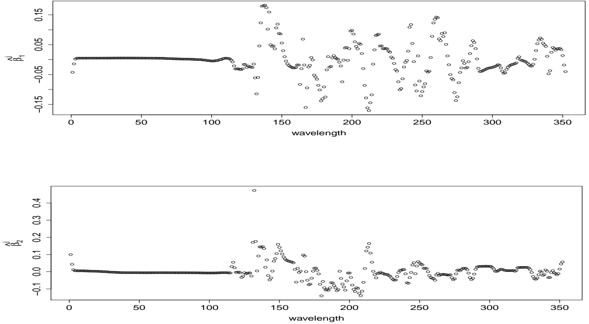
Figure 10: Final first and second EDR directions obtained with SIRd on all the blocks.
