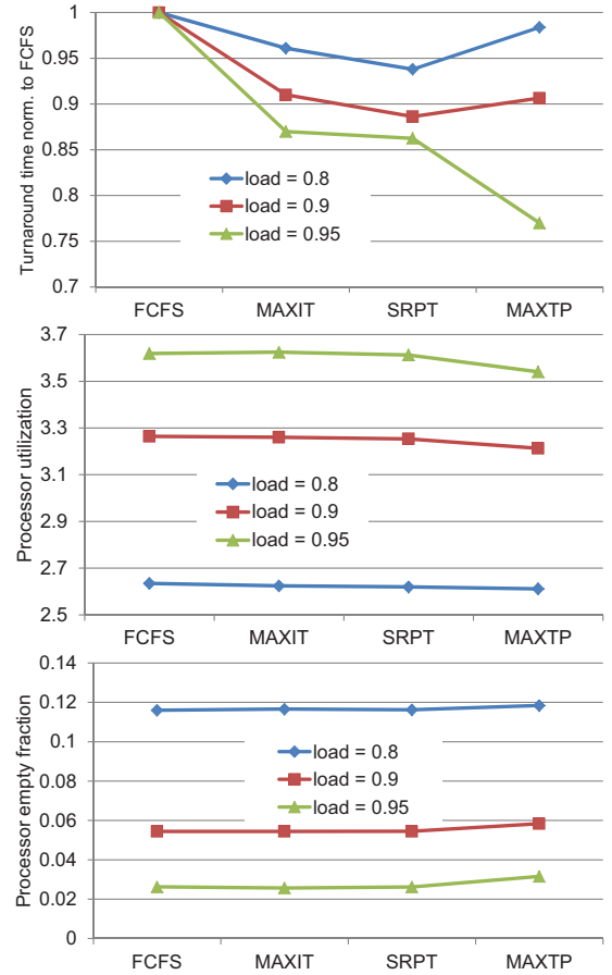
Fig. 5. Turnaround time, processor utilization and processor empty fraction for the FCFS, MAXIT, SRPT and MAXTP scheduler, and three different loads (relative to the FCFS maximum throughput).
